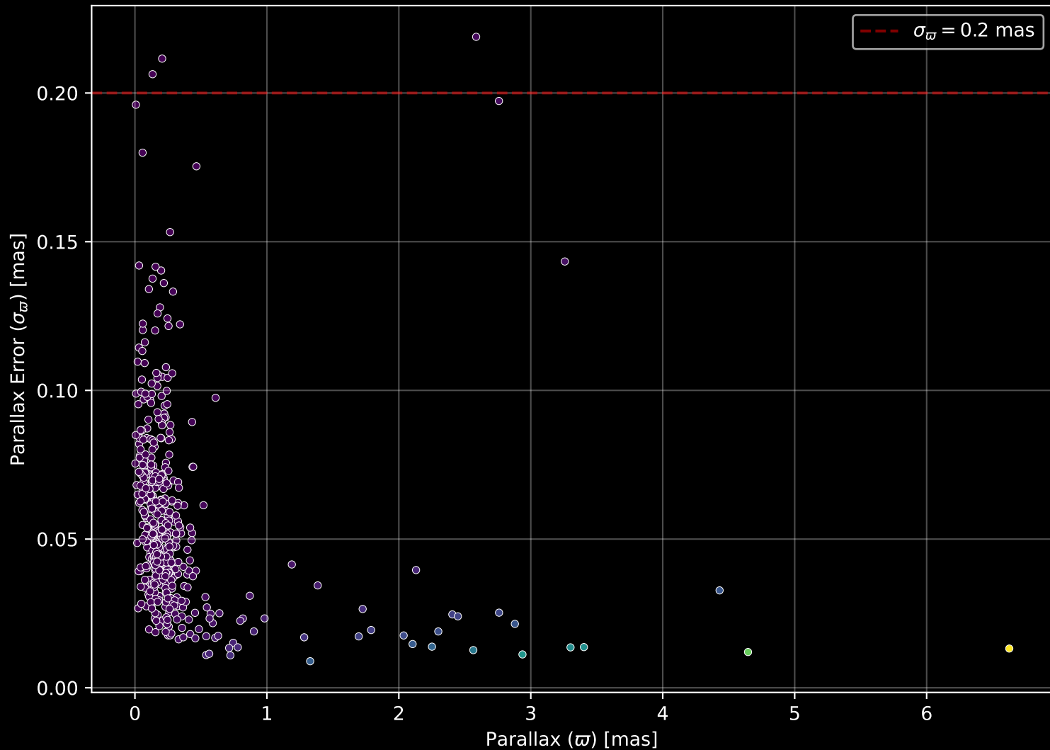
APOGEE DR17 Field: [259+00] Parallax Quality (n= 455)
