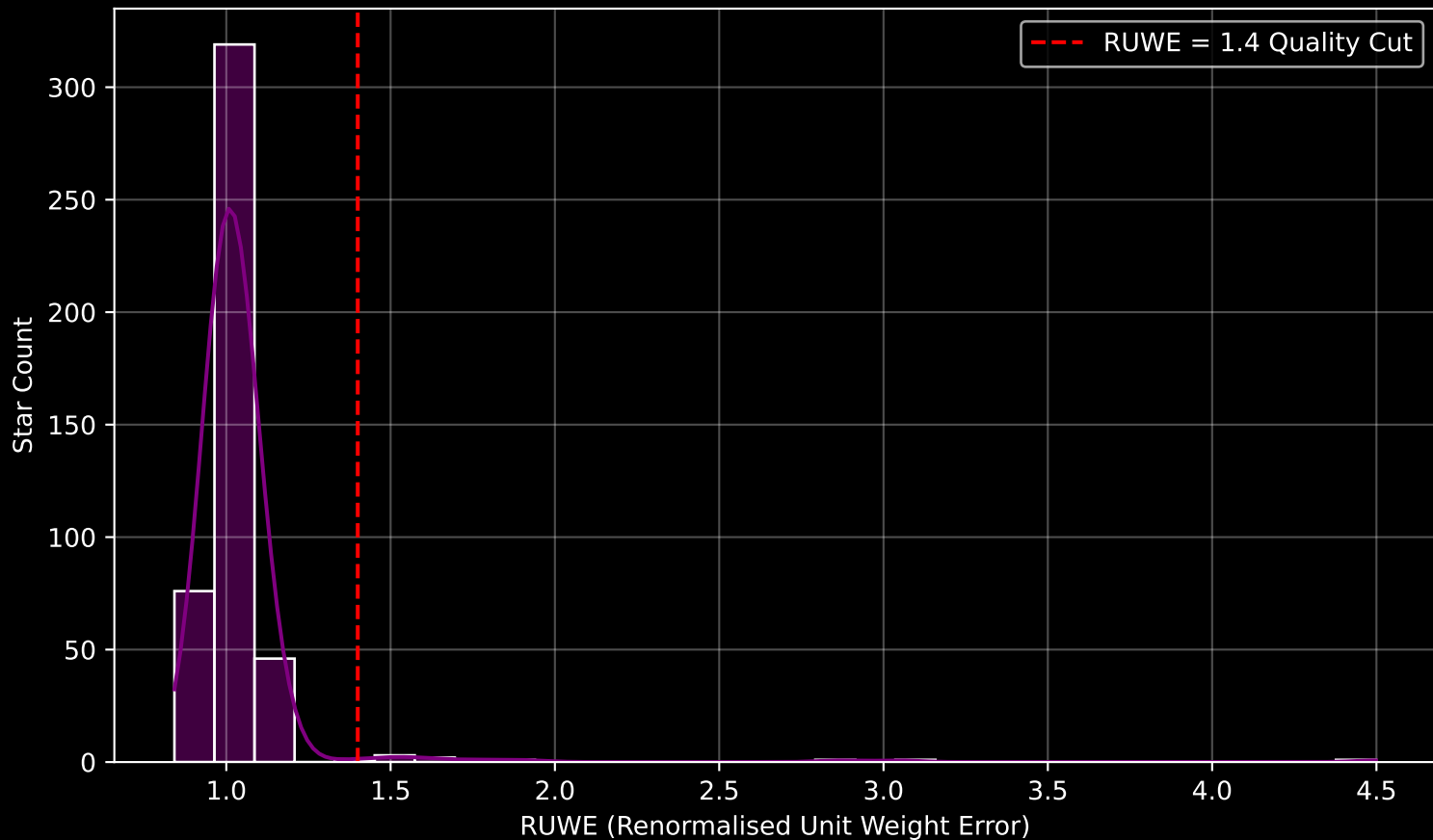
GAPOGEE DR17 Field [259+00] RUWE Distribution (n= 452)
