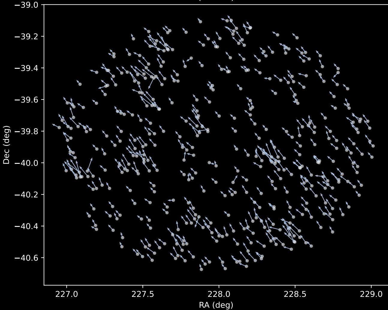
APOGEE DR17 Cluster 1 Proper Motion Vectors (n=435)
