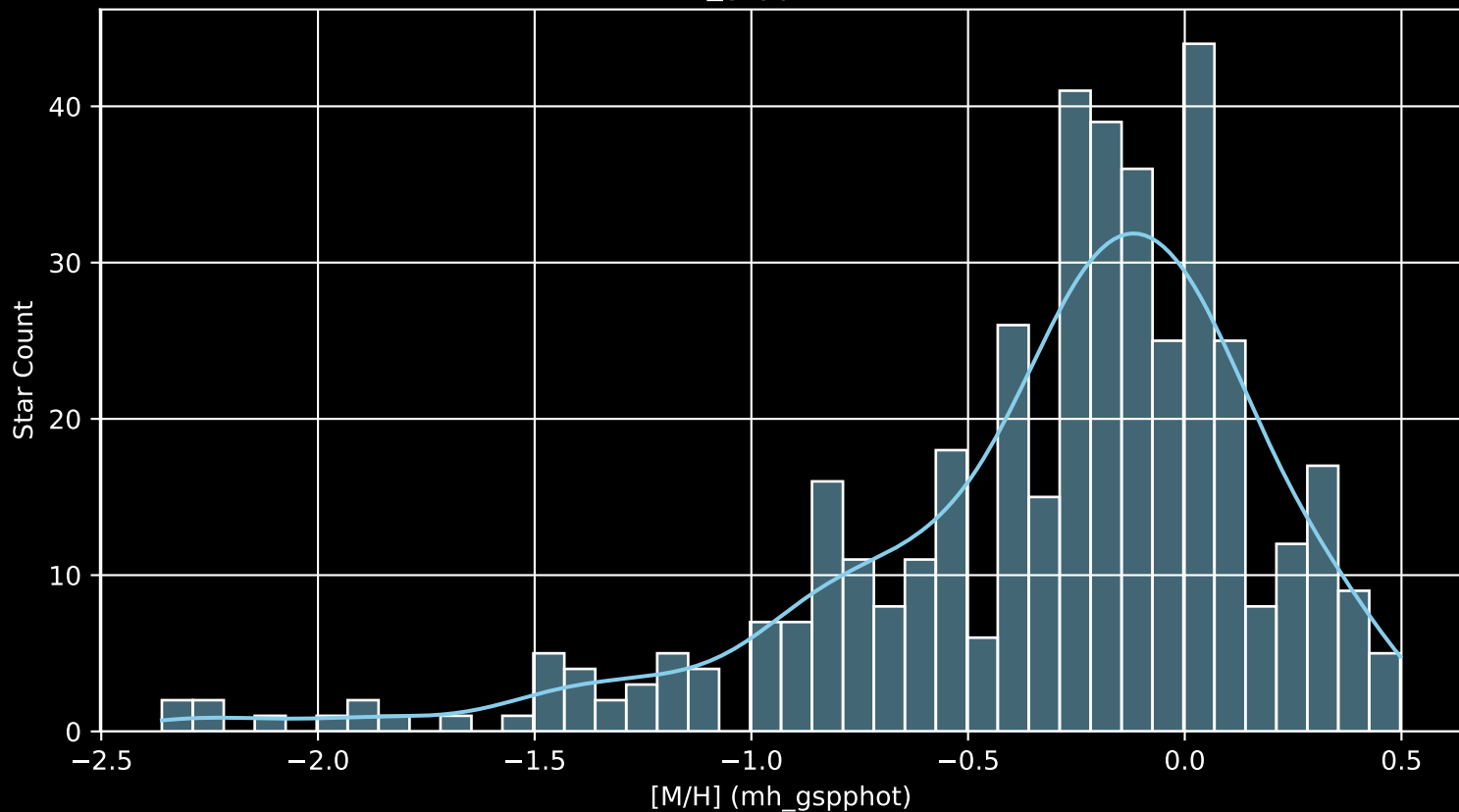
APOGEE DR17 Field: [259+00 [M/H] (mh_gspphot) (n= 420)
