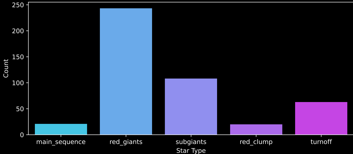
APOGEE DR17 Field: [259+00] Count plot of Star Type
