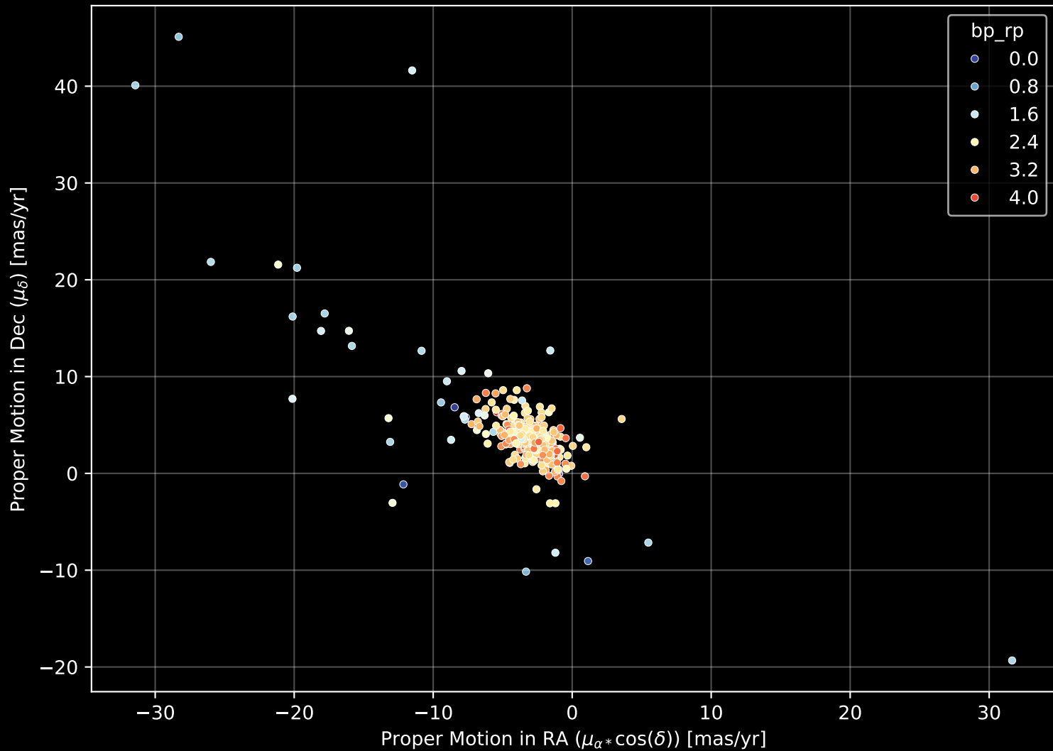
APOGEE DR17 Field: [259+00] Proper Motion Diagram (n= 455)
